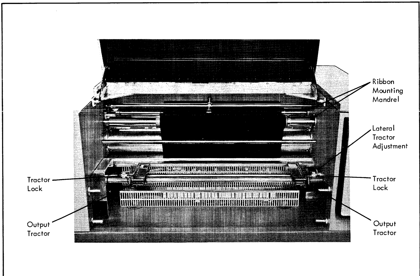
Figure 3. Printer Mechanism, Front View
