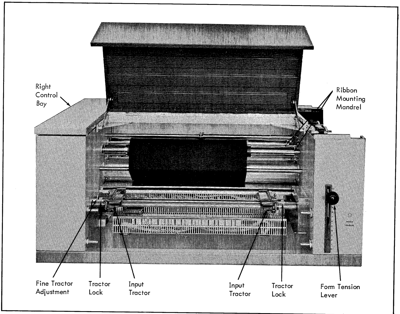
Figure 4. Printer Mechanism, Rear View
