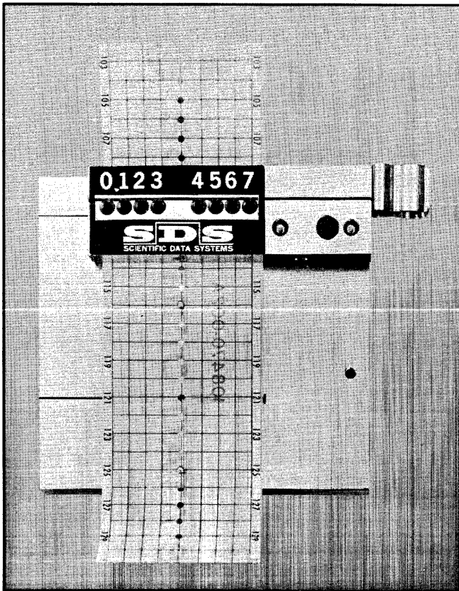
Figure 8. Tape Alignment in VFU Tape Punch
