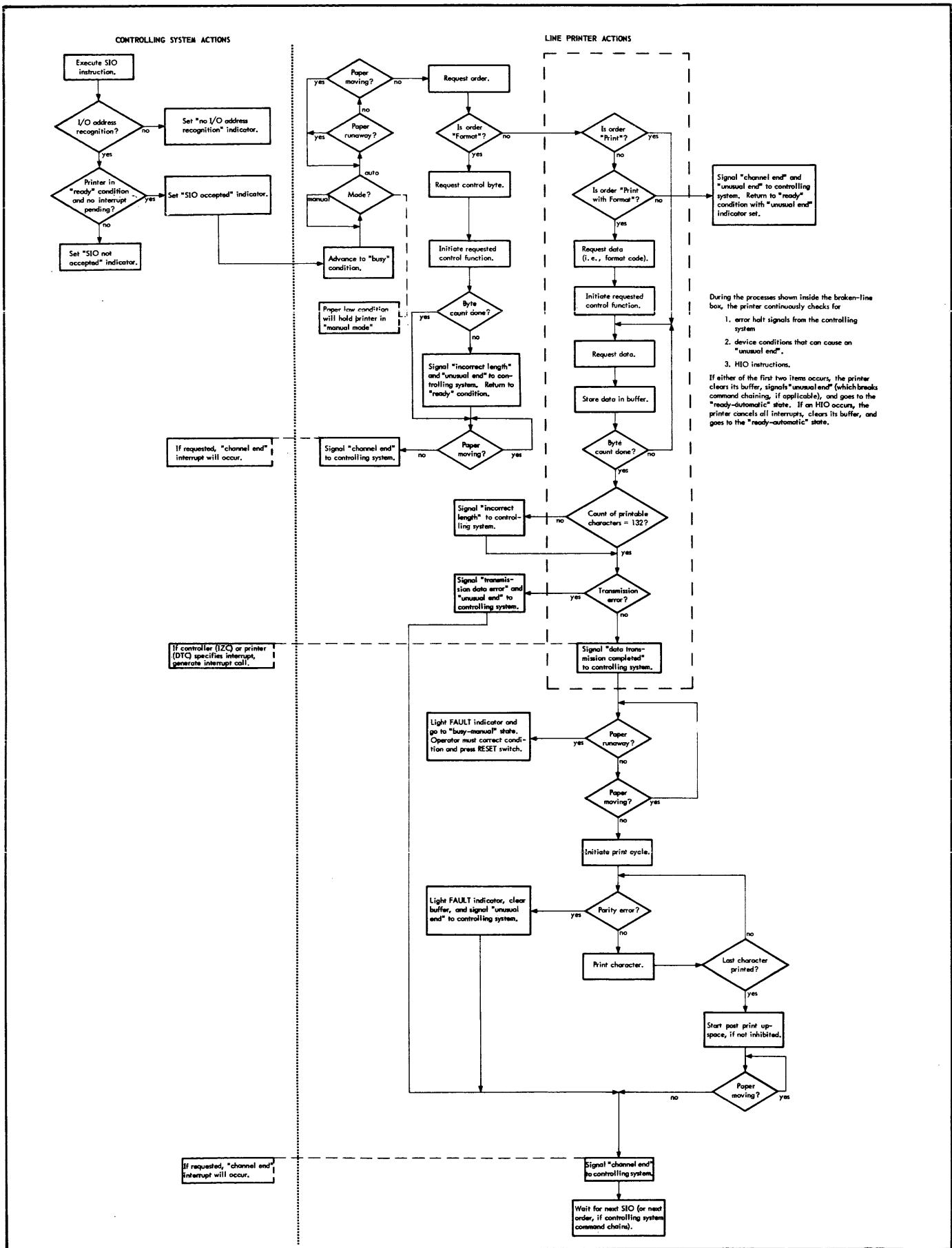
Figure 1. Controlling System/Line Printer Actions
